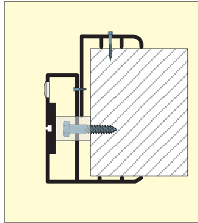
2. PK2 aluminium Foder 70-130 mm
