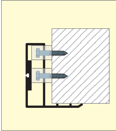
1. PK1 aluminium Foder end. fram
